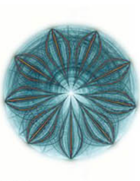
Z920/0373 Atlantic spotted solphin, wavelet graph
