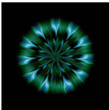
Z892/0848 Chipping sparrow song, wavelet graph
